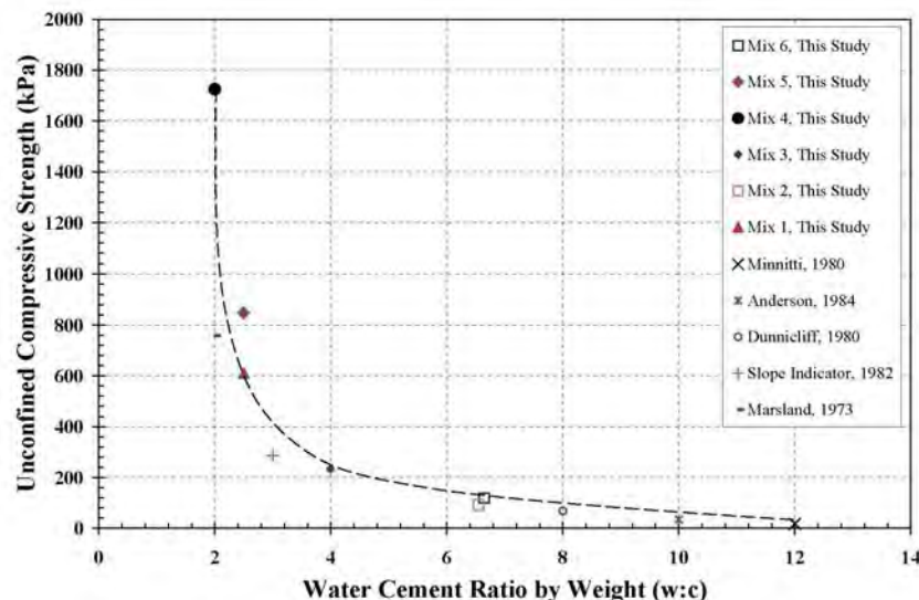
Figure 4. Variation of unconfined compressive strength versus water:cement ratio.
