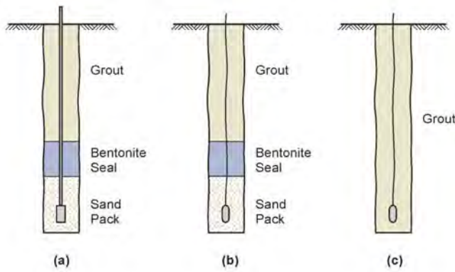
Figure 1(a). Traditional standpipe piezometer with sand pack. Figure 1(b). Diaphragm piezometer with sand pack. Figure 1(c). Fully-grouted piezometer.
